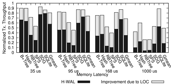
Fig. 9: Sensitivity to Memory Latency.
