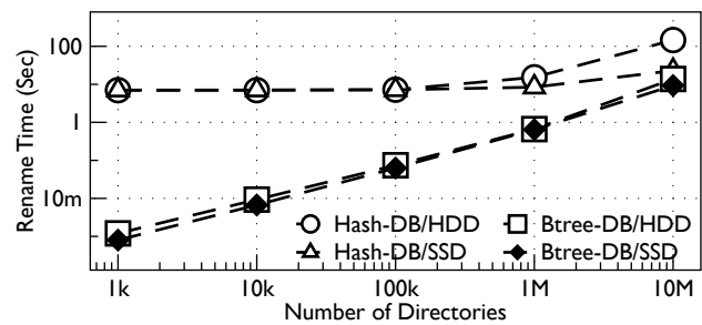
Figure 14: Rename Overhead.
