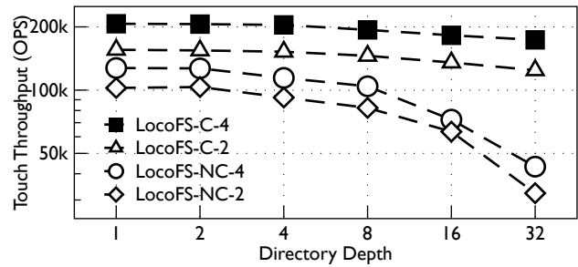
Figure 13: Sensitivity to the Directory Depth. LocoFS-C and LocoFS-NC respectively stand for LocoFS with cache enabled and disabled. 2 and 4 stand for the number of metadata servers.
